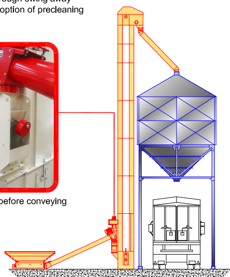
Reception through swing away hopper, with option of precleaning
